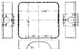
Figs. 958-961. Steam Chest Casing. Atlantic (4-1-2) Locomotive. Pennsylvania Railroad.
